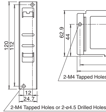
PS9Z-5R1B Panel Mounting Bracket
