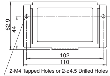
PS9Z-5R2B Panel Mounting Bracket
