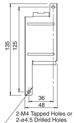
PS9Z-5R1E Panel Mounting Bracket
