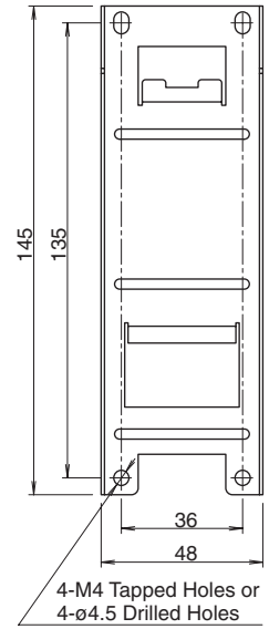
PS9Z-5R1G Panel Mounting Bracket
