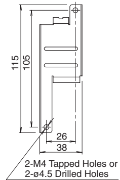
PS9Z-5R1C Panel Mounting Bracket
