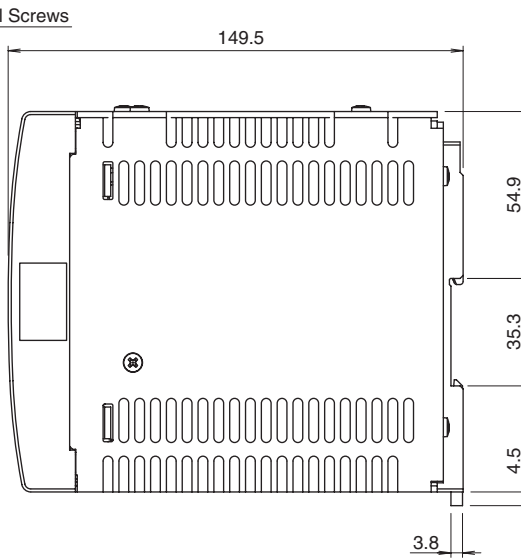
PS9Z-5R1G Panel Mounting Bracket
