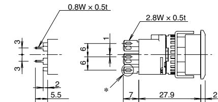
PC Board Terminal
