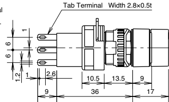
Solder/Tab Terminal
