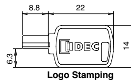
Logo Stamping
